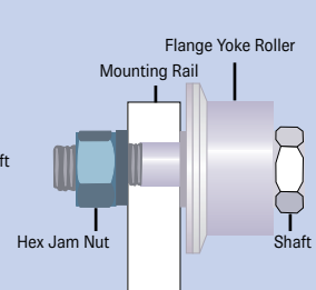
Through-Hole Mount Yoke Type
