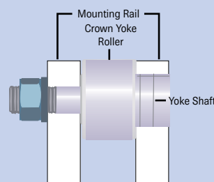
Captured Mount Yoke Type
